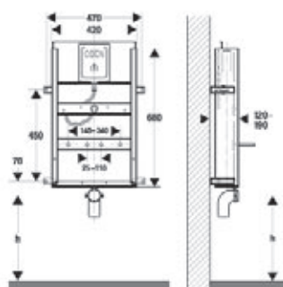
MONTAGE-SET Urinelement
