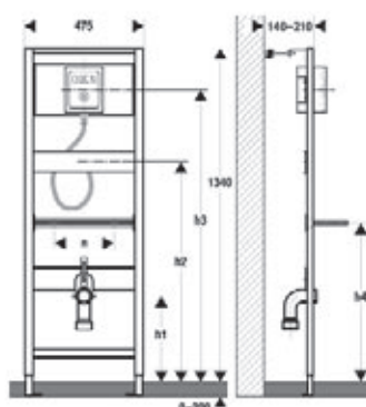
DUPLO XS Urinelement
